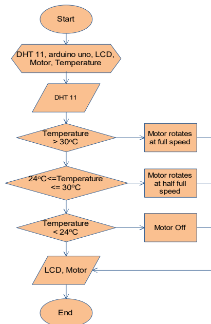
FIGURE 5. Flowchart of DHT11 circuit, LCD and DC Motor to Arduino
